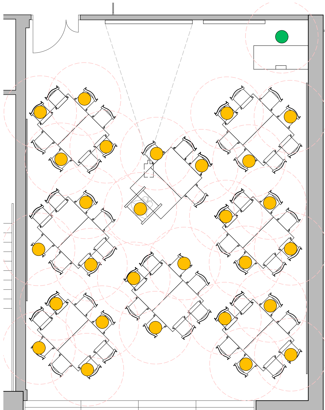
Room 2.F.11 - First Floor - Social Distancing 1:50 @ A3
